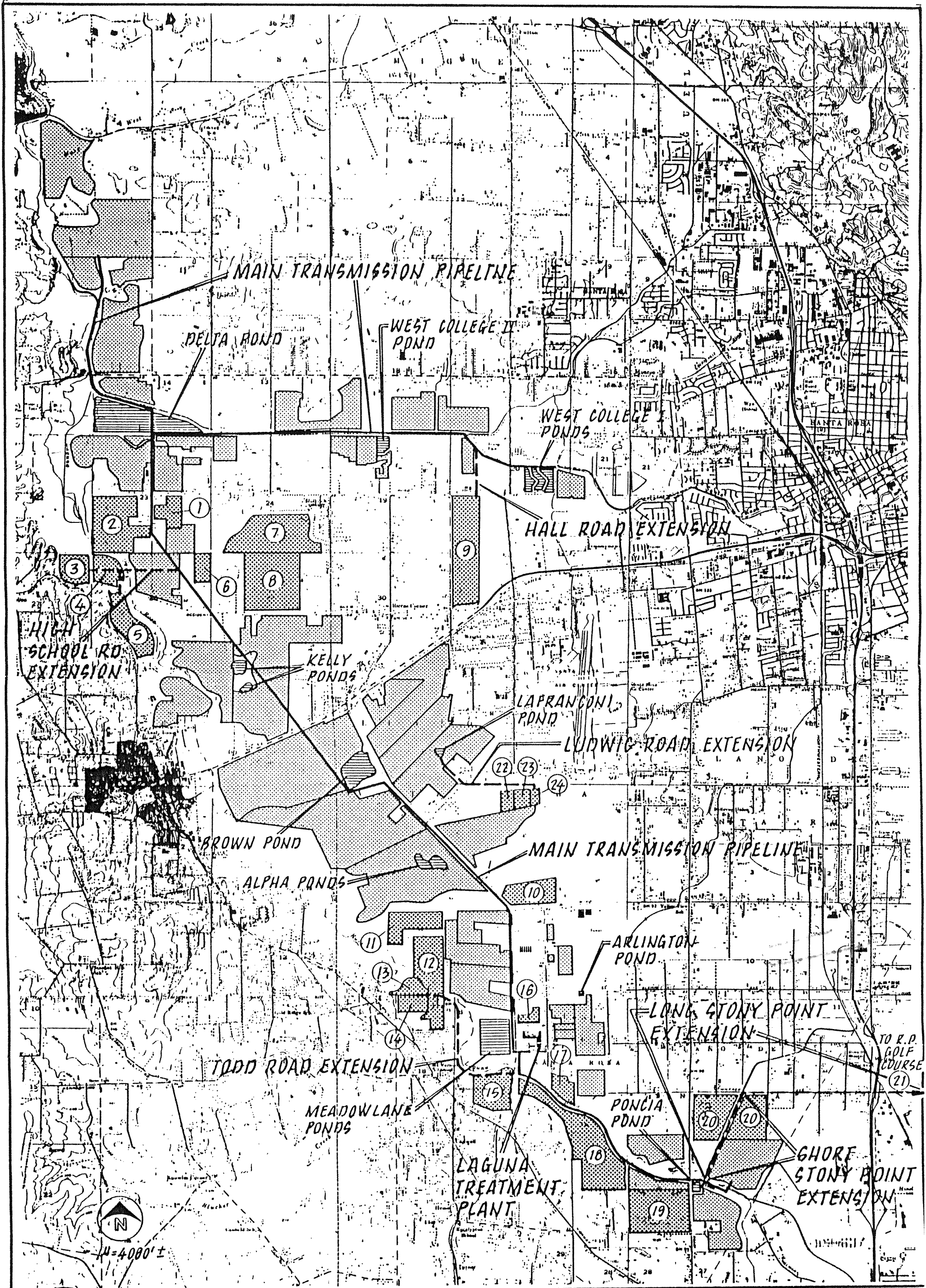
FIGURE 1 EXISTING IRRIGATED AREAS AND POSSIBLE EXPANSION SITES WASTEWATER DISPOSAL SYSTEM
